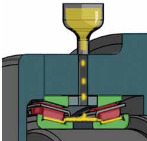
Lubrication by dripping
