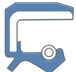
Double lips with spring
