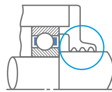
Groove in the box
