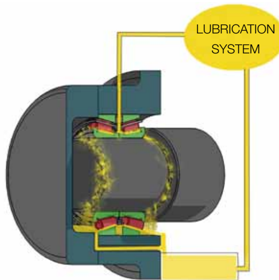
Oil circulation
