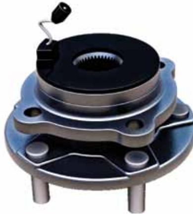
Active sensor + multi-pole encoder
