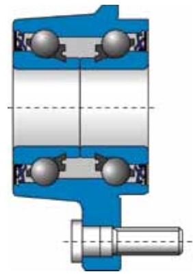
Rotating Inner Ring - driven wheels
