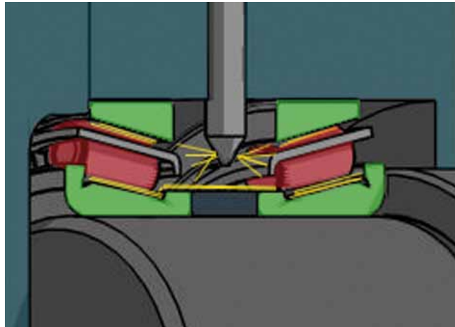
Injection of oil
