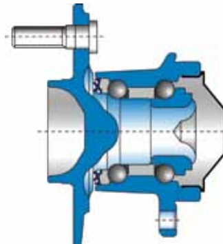
Rotating Inner Ring - non-driven wheels
