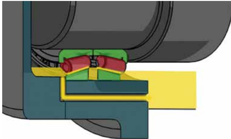
Oil bath
