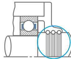
Groove in the box and axis
