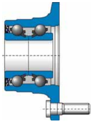
Rotating Inner Ring - non-driven wheels
