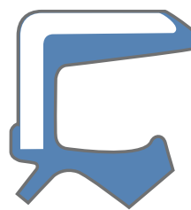
Double lips without spring
