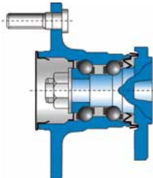
Rotating Outer Ring - non-driven wheels
