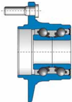
Rotating Outer Ring - non-driven wheels
