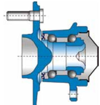
Rotating Inner Ring - driven wheels
