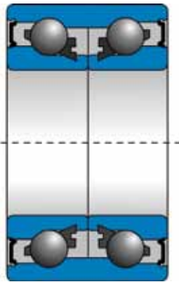
Double Row Angular Contact Ball Bearing
